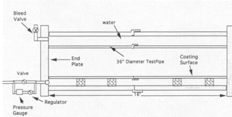
Figure 1. Hydrostatic Pressure Test Chamber Used for Evaluating the Application and Performance of Coatings on Concrete Surface
