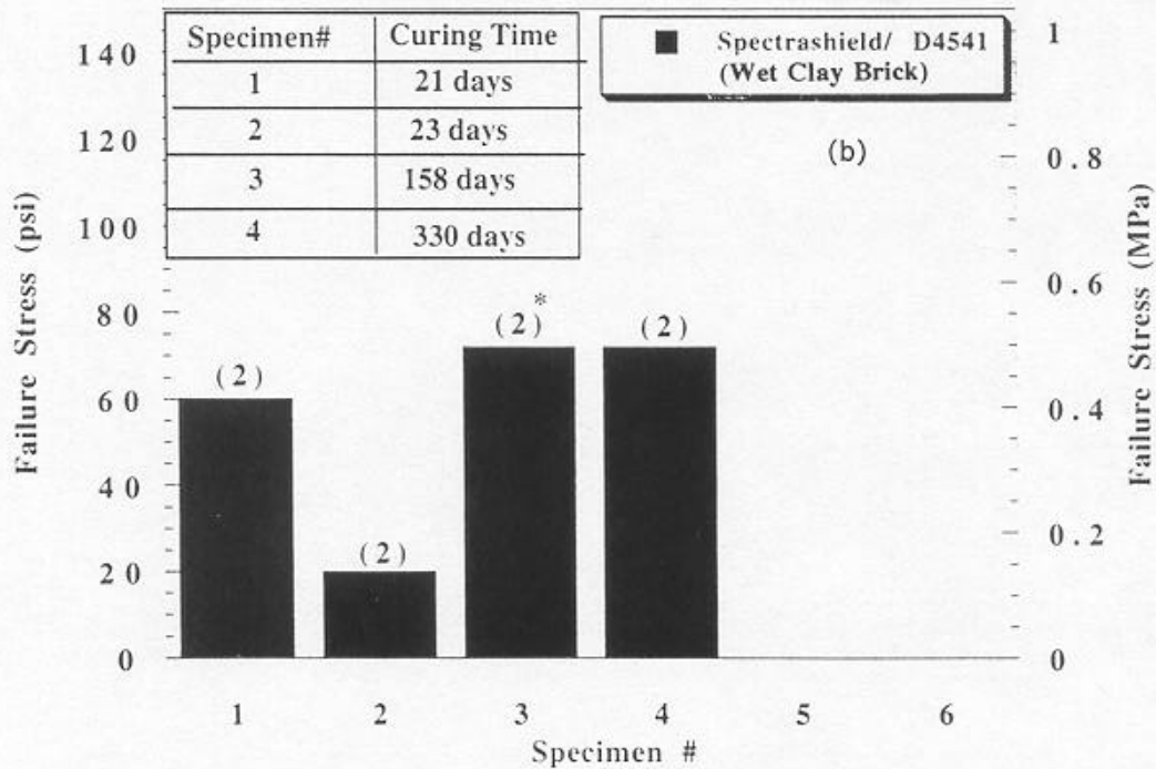
Figure D3. Bonding Strength of SPECTRASHIELD LINER with Clay Brick and Types of Failures During ASTM D4541-85 Tests (a) Dry and (b) Wet Clay Bricks
