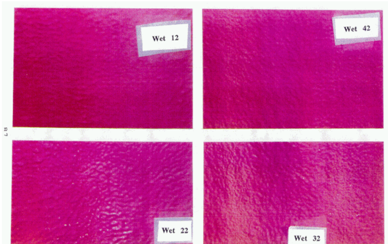
Figure B2. Middle Section of the Concrete Pipe Coated with SPECTRASHIELD LINER (Wet Coating) After Five Months of Testing
