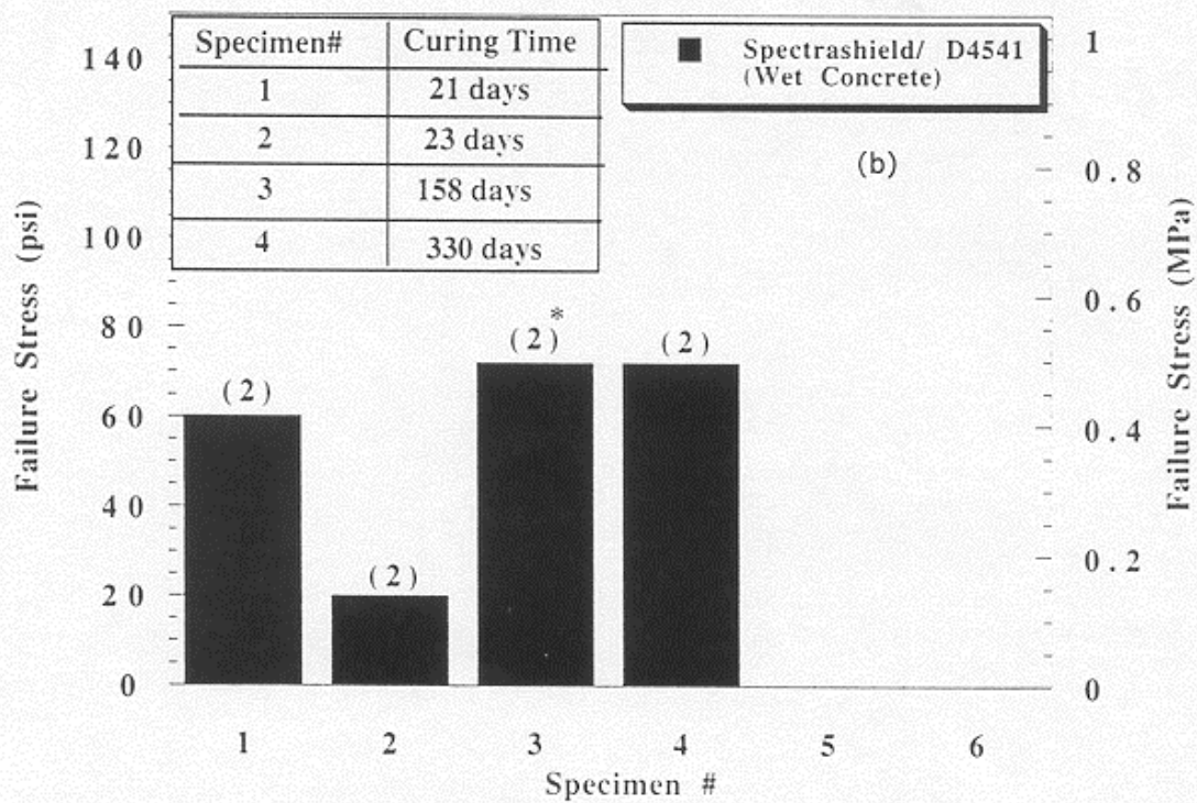
Figure D2. Bonding Strength of SPECTRASHIELD LINER with Concrete and Types of Failures During ASTM D4541-85 Tests (a) Dry and (b) Wet Concrete
