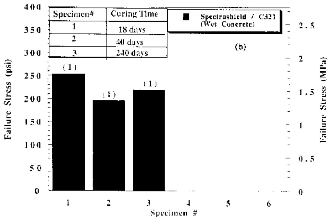
Figure D5. Bonding Strength of SPECTRASHIELD LINER with Concrete and Types of Failures During ASTM C321-94 Tests (a) Dry and (b) Wet Concrete
