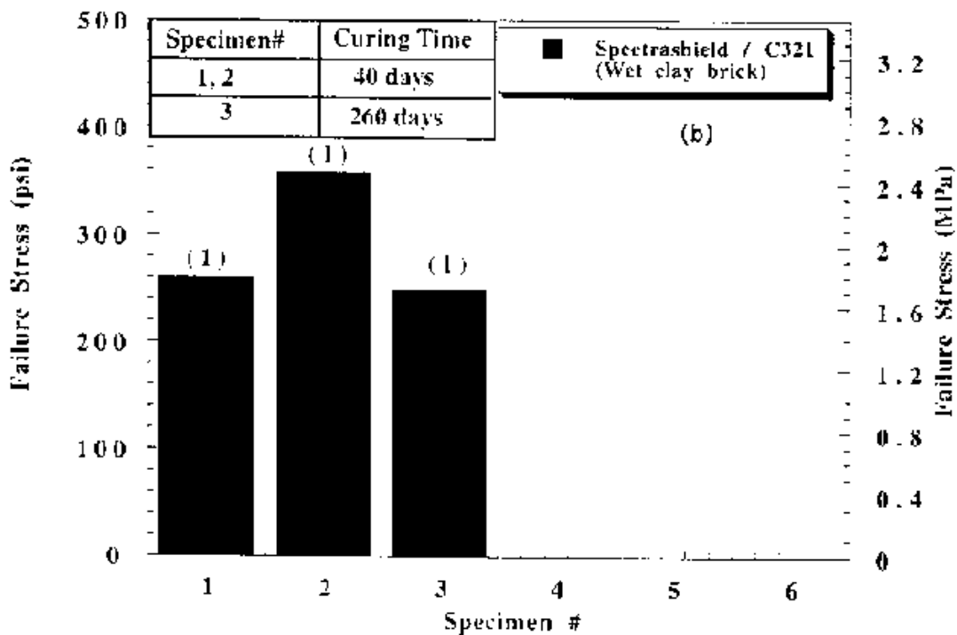
Figure D6. Bonding Strength of SPECTRASHIELD LINER with Clay Brick and Types of Failures During ASTM C321-94 Tests (a) Dry and (b) Wet Clay Bricks
